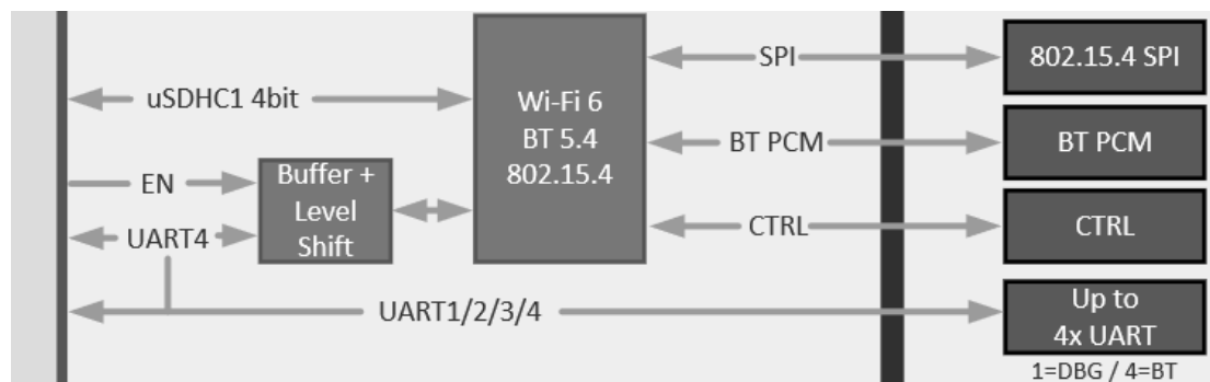
Figure 3: DART-MX8M-PLUS Wi-Fi & BT Internal Connection
