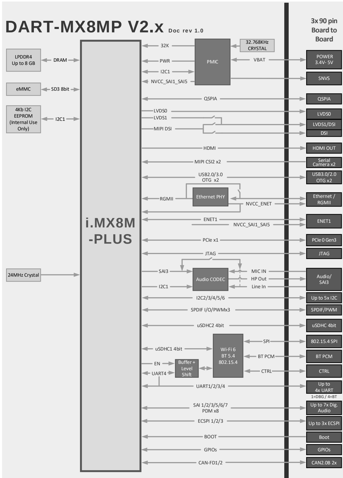
Figure 1 : DART-MX8M-PLUS Block Diagram
